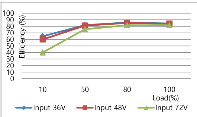
COP7S-48-12 EFFICIENCY CURVE VS LOAD AT25°C
