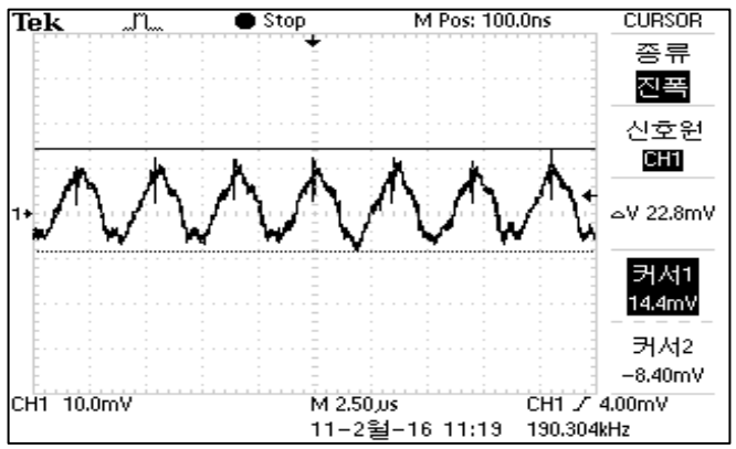
COP7S-24-05 RIPPLE & NOISE VIN=24VDC, MAX-LOAD AT25°C
