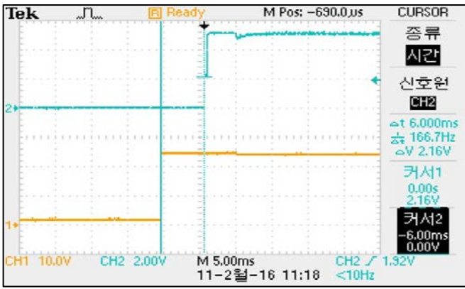
COP7S-24-05 TURN-ON TIME VIN=24VDC, MAX-LOAD AT25°C
