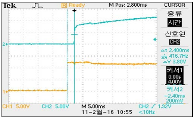
COP7S-12-12 TURN-ON TIME VIN=12VDC, MAX-LOAD AT25°C
