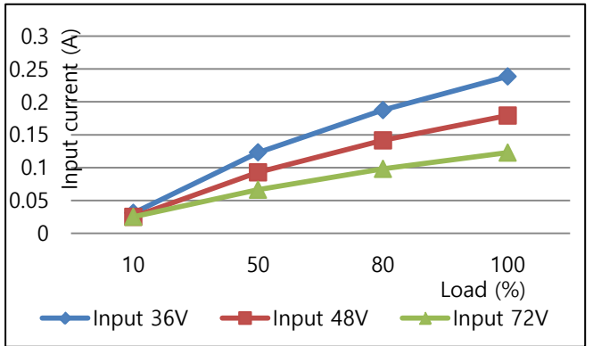
COP7S-48-12 INPUT CURRENT CURVE VS LOAD AT25°C
