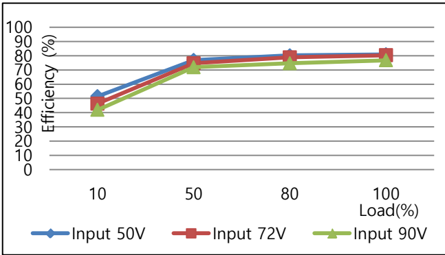
COP7S-72-12 EFFICIENCY CURVE VS LOAD AT25°C
