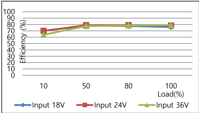
COP7S-24-05 EFFICIENCY CURVE VS LOAD AT25°C
