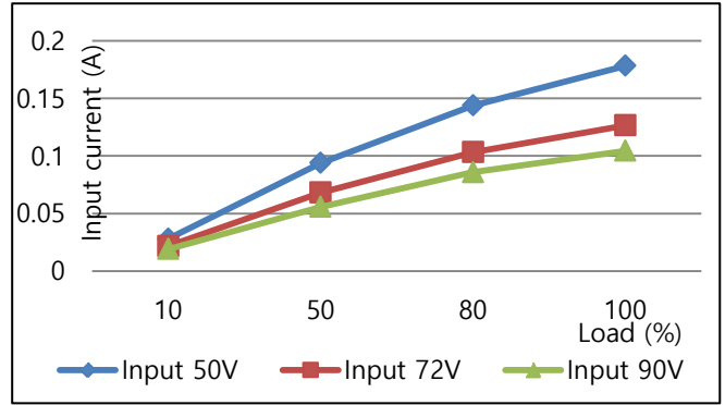
COP7S-72-12 INPUT CURRENT CURVE VS LOAD AT25°C
