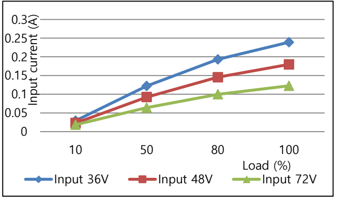
COP7S-48-05 INPUT CURRENT CURVE VS LOAD AT25°C
