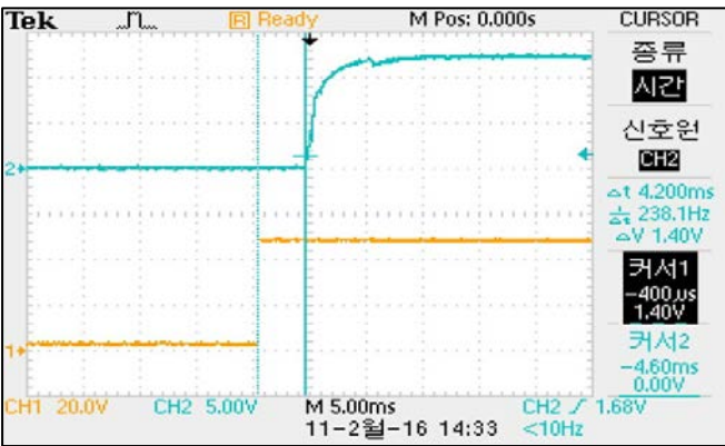
COP7S-48-12 TURN-ON TIME VIN=48VDC, MAX-LOAD AT25°C
