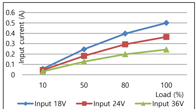
COP7S-24-12 INPUT CURRENT CURVE VS LOAD AT25°C
