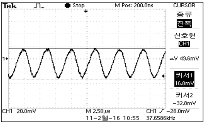
COP7S-12-12 RIPPLE & NOISE VIN=12VDC, MAX-LOAD AT25°C
