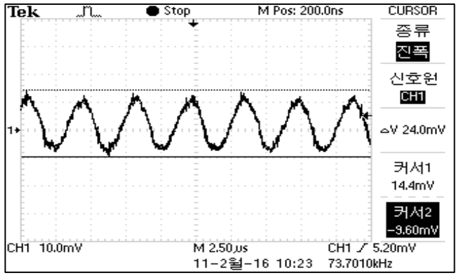
COP7S-12-05 RIPPLE & NOISE VIN=12VDC, MAX-LOAD AT25°C
