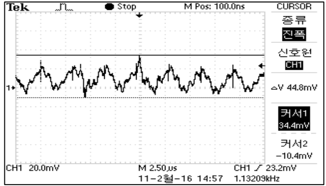
COP7S-72-12 RIPPLE & NOISE VIN=72VDC, MAX-LOAD AT25°C
