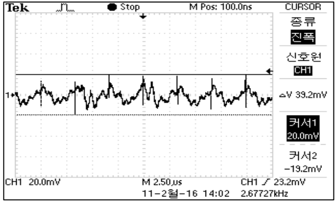
COP7S-48-05 RIPPLE & NOISE VIN=48VDC, MAX-LOAD AT25°C
