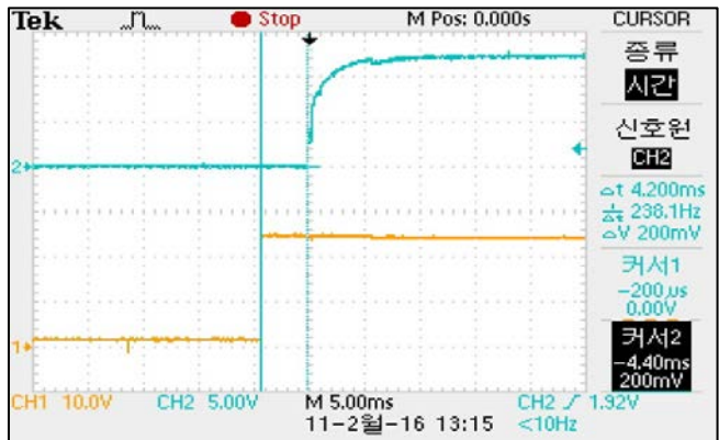
COP7S-24-12 TURN-ON TIME VIN=24VDC, MAX-LOAD AT25°C
