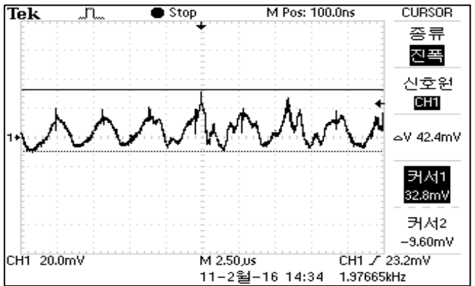
COP7S-48-12 RIPPLE & NOISE VIN=48VDC, MAX-LOAD AT25°C
