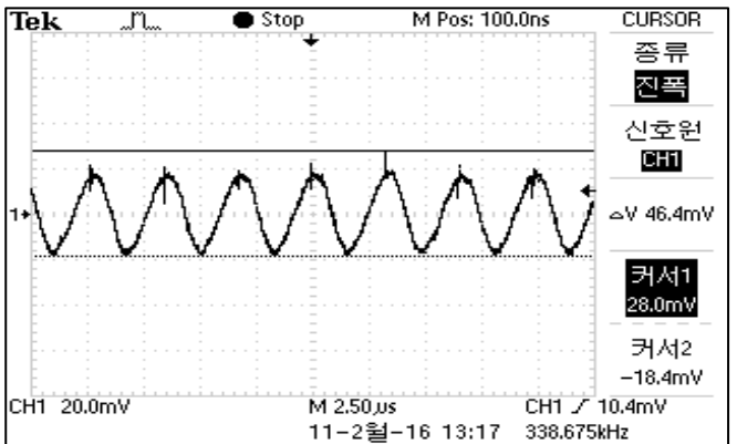
COP7S-24-12 RIPPLE & NOISE VIN=24VDC, MAX-LOAD AT25°C
