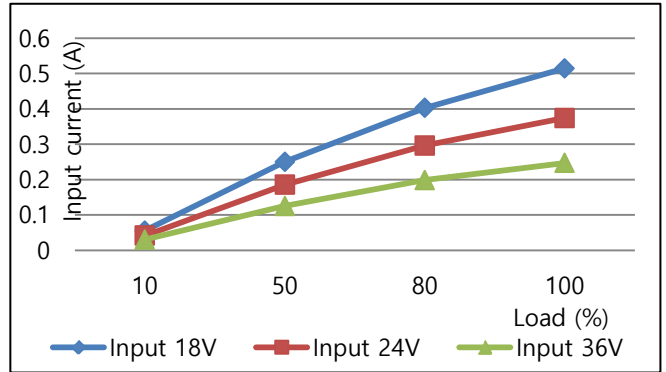
COP7S-24-05 INPUT CURRENT CURVE VS LOAD AT25°C
