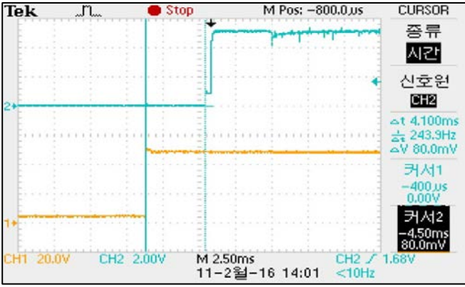
COP7S-48-05 TURN-ON TIME VIN=48VDC, MAX-LOAD AT25°C
