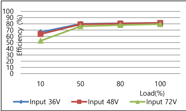
COP7S-48-05 EFFICIENCY CURVE VS LOAD AT25°C
