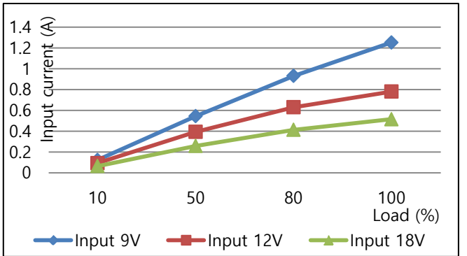
COP7S-12-05 INPUT CURRENT CURVE VS LOAD AT25°C
