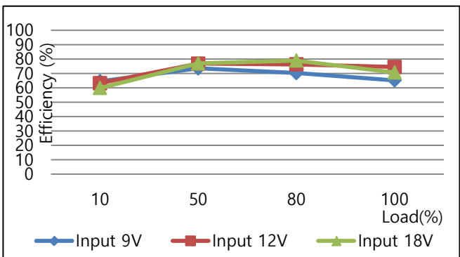
COP7S-12-12 EFFICIENCY CURVE VS LOAD AT25°C
