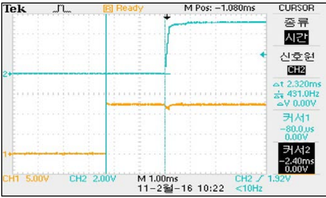
COP7S-12-05 TURN-ON TIME VIN=12VDC, MAX-LOAD AT25°C
