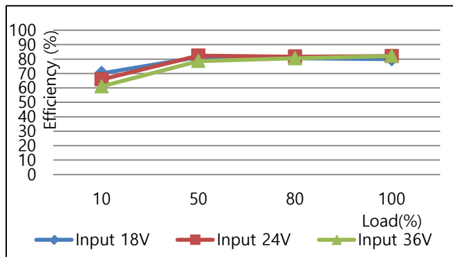
COP7S-24-12 EFFICIENCY CURVE VS LOAD AT25°C
