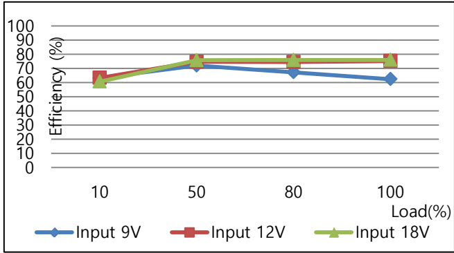
COP7S-12-05 EFFICIENCY CURVE VS LOAD AT25°C
