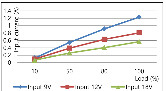
COP7S-12-12 INPUT CURRENT CURVE VS LOAD AT25°C
