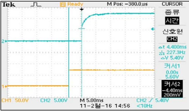
COP7S-72-12 TURN-ON TIME VIN=72VDC, MAX-LOAD AT25°C
